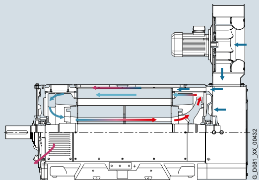
1LQ1/1MQ1 force-ventilated motors – enclosed version
