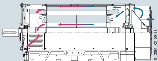
1LL1 self-ventilated motors – open version
