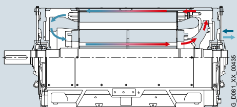
1LH1/1MH1 water-cooled motors with water-jacket cooling
