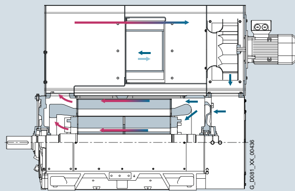
1LN1/1MN1 water-cooled motors with air-to-water heat exchanger
