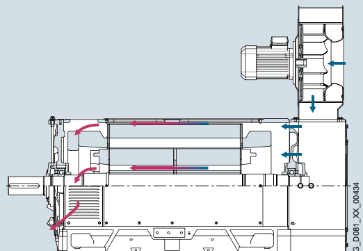
1LP1 forced-ventilated motors – open version
