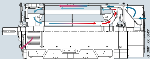
1LM1/1MM1 self-ventilated motors – enclosed version
